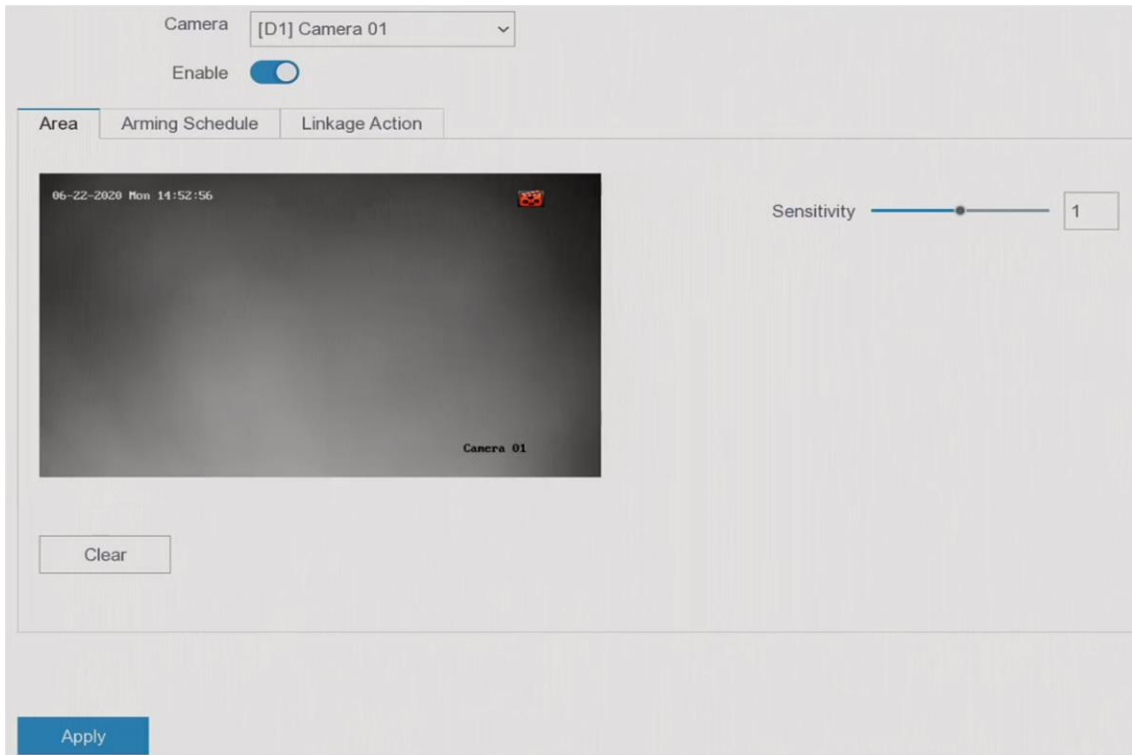
Figure 6-15 Video Tampering
