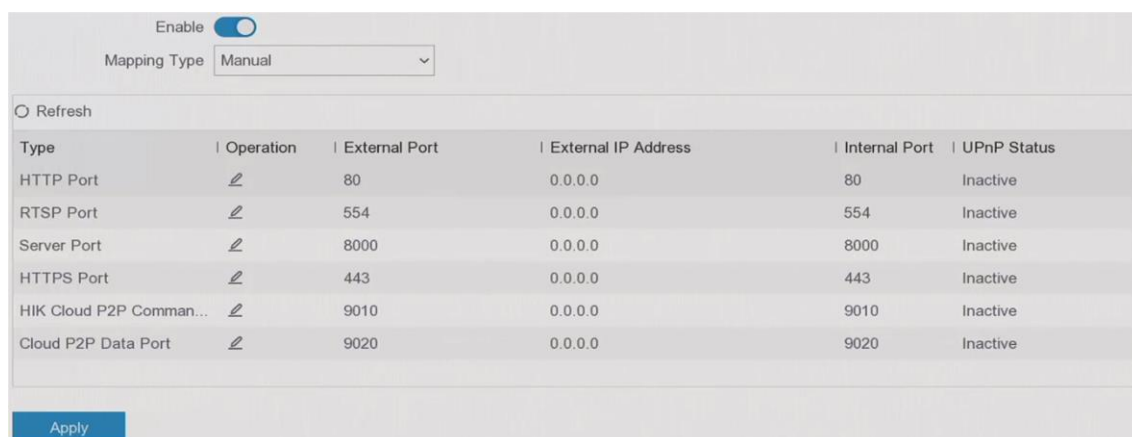
Figure 6-5 NAT
