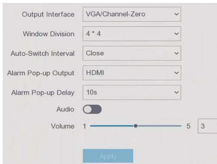
Figure 6-2 Live View-General
