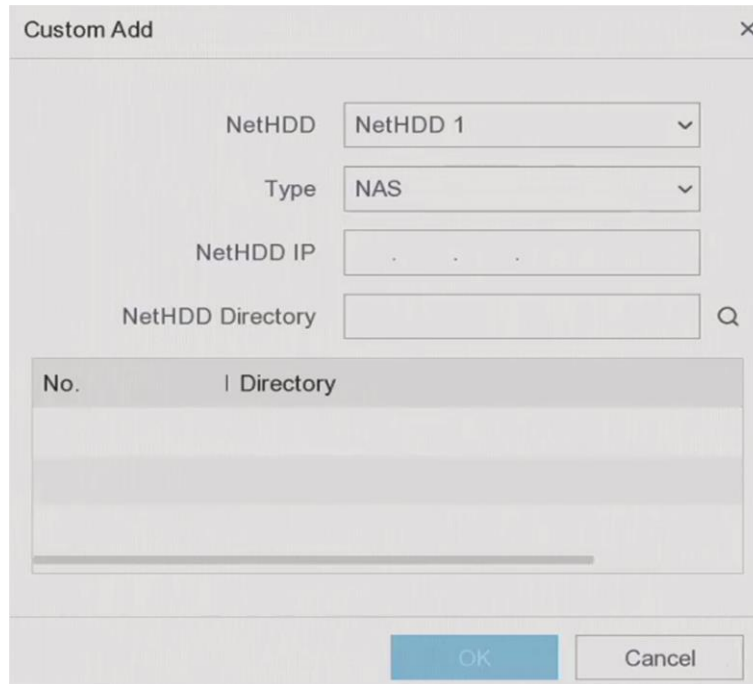
Figure 5-11 Add NetHDD
