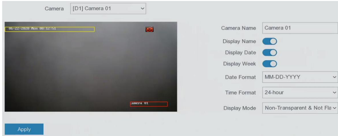
Figure 5-9 OSD
