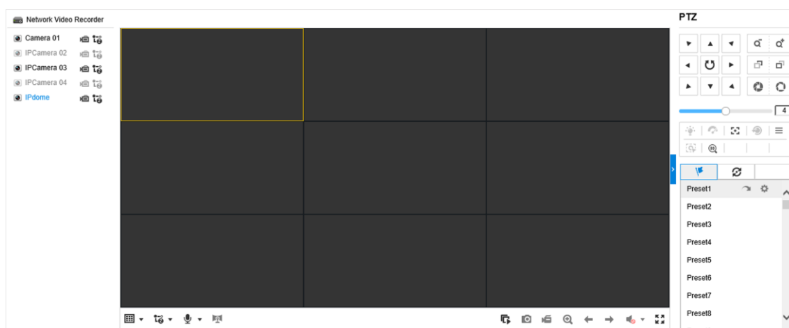
Figure 9-2 Live View
