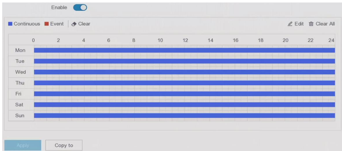
Figure 5-12 Recording Schedule
